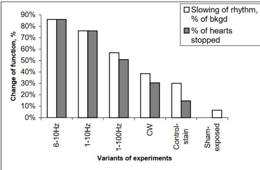
Figure 5: Heart rate variability and arrests in isolated frog hearts irradiated with RF in continuous mode (CW) and with (ELF) pulse modulation varying 1-100 Hz (reproduced from Maslov and Grigoriev, 2003, p.67)
